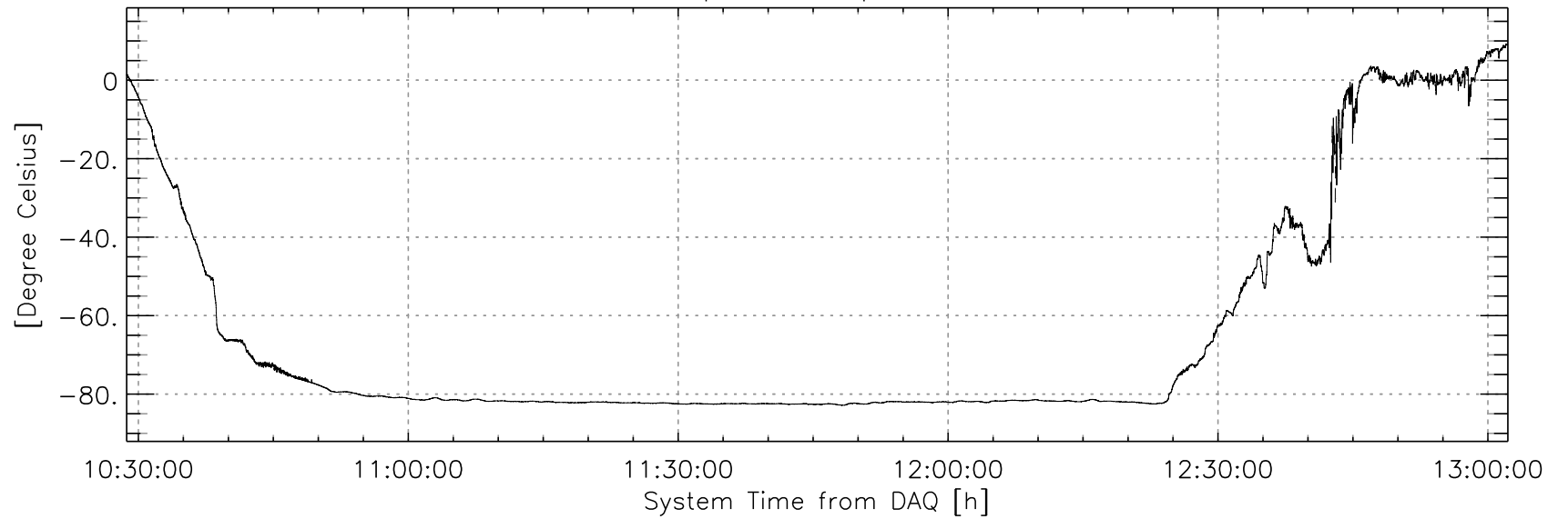
Dewpoint Temperature
