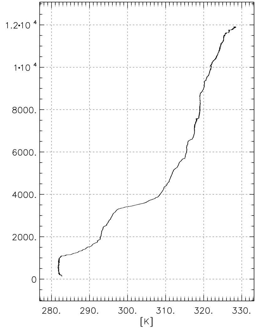
Potential Temperature
