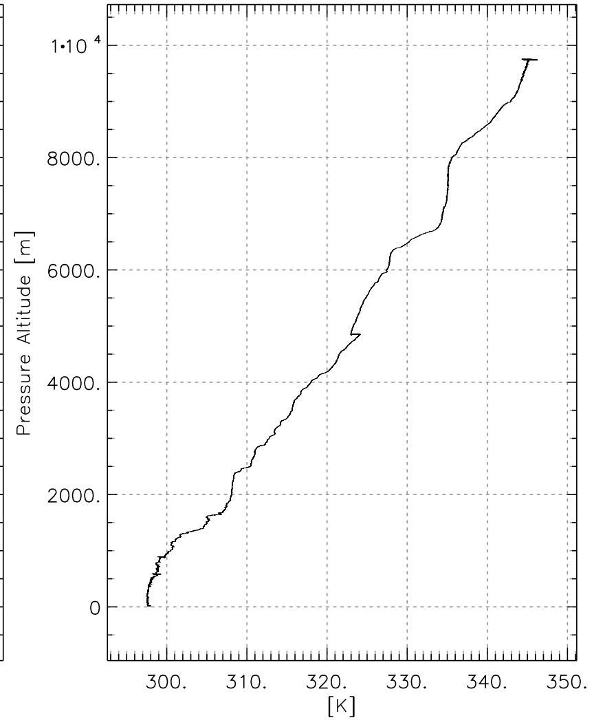
Potential Temperature
