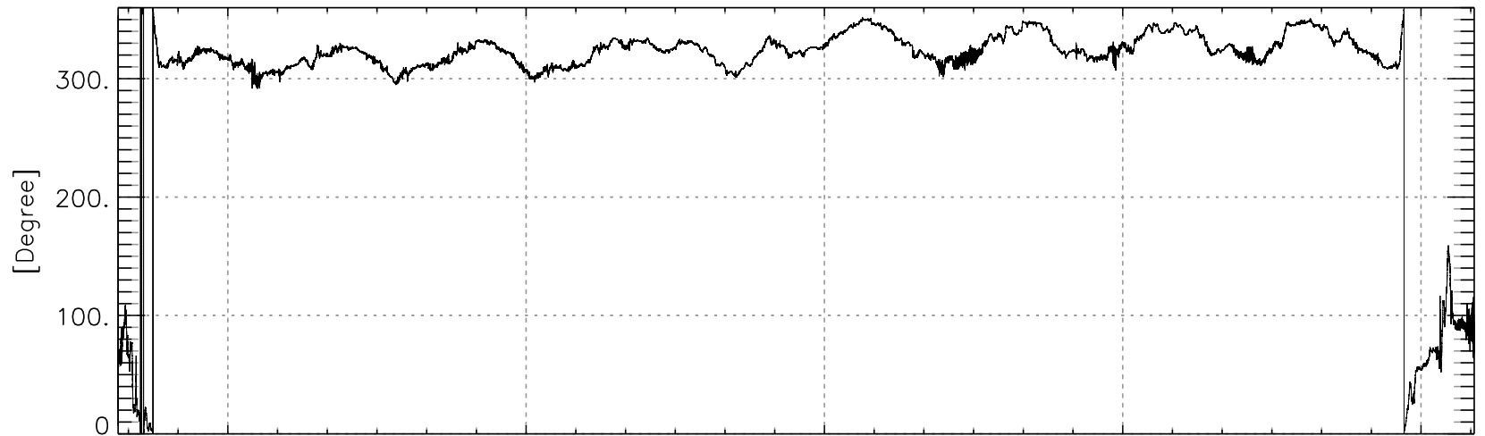
Horizontal Wind Direction
