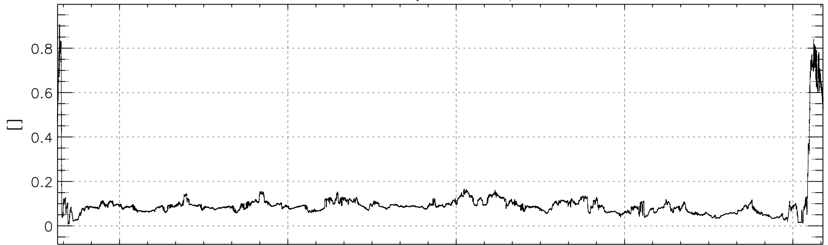
Relative Humidity with Respect to Ice
