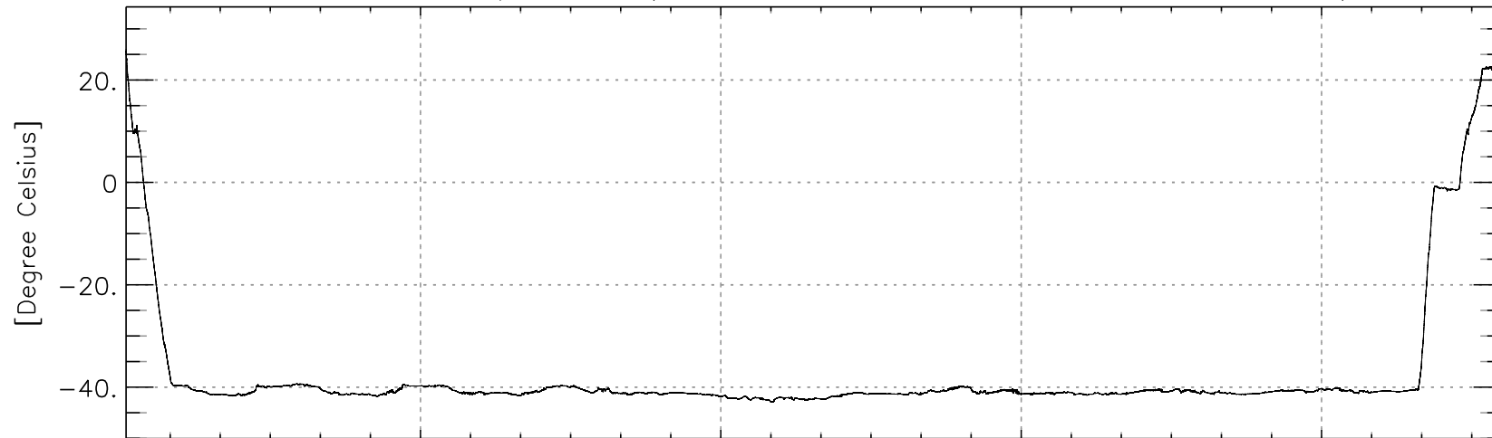
Static Air Temperature (from BDY-TTQ, anti-ice was not activated)
