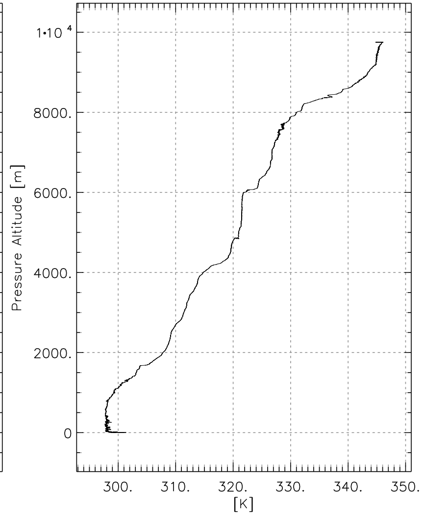
Potential Temperature
