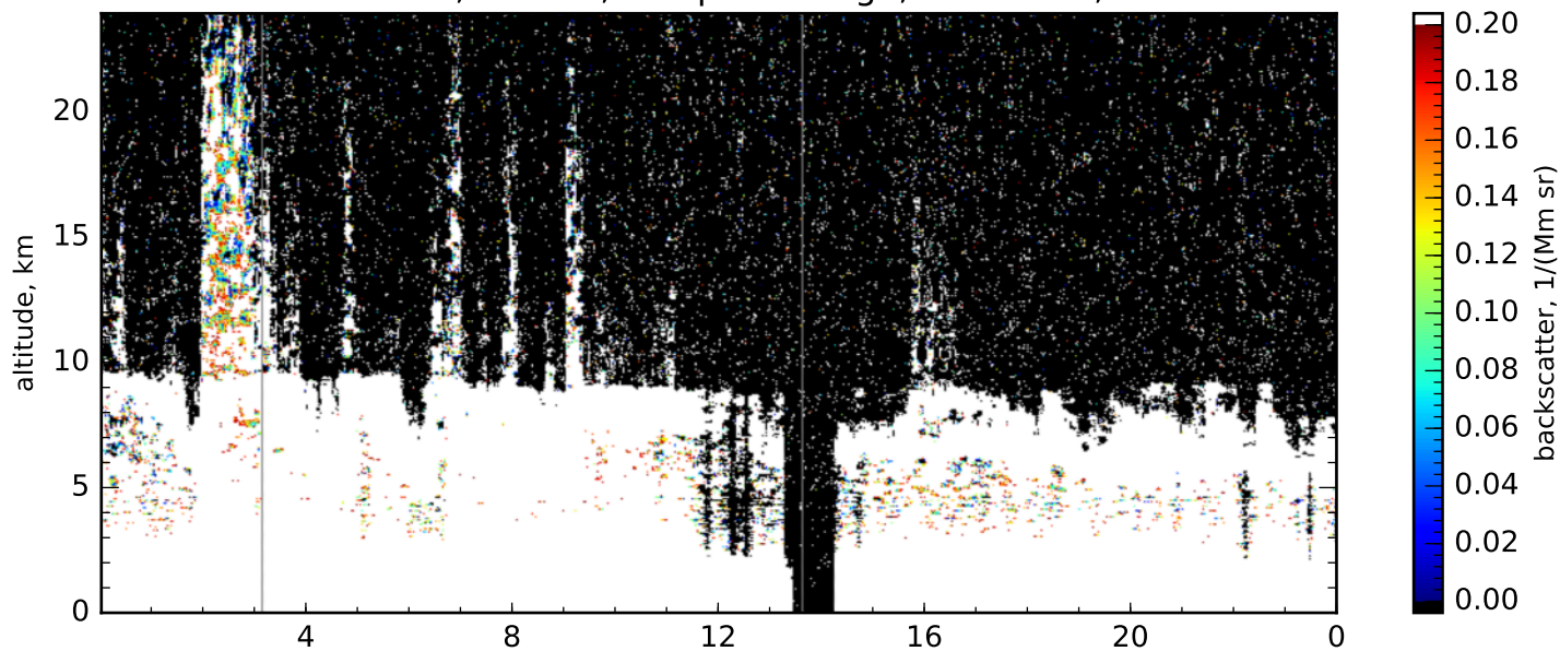
Particle backscatter, 355nm, complete range, res.: 600s, 60m-1020m
