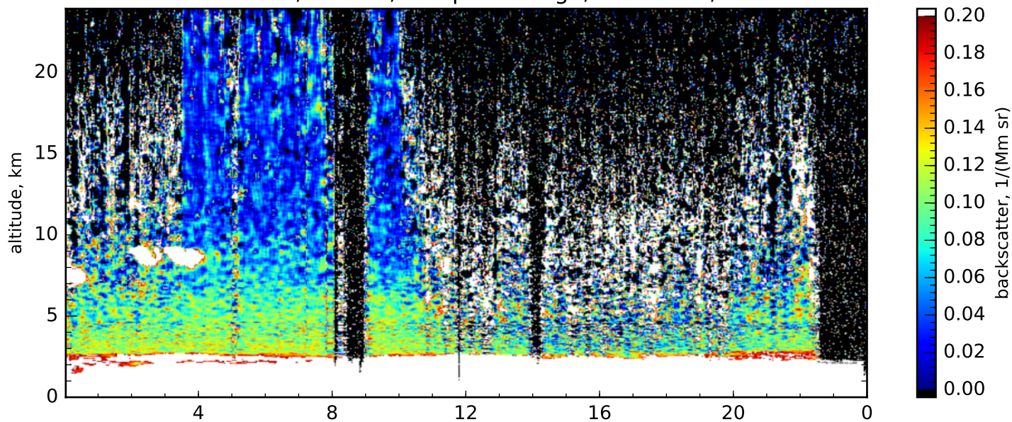
Particle backscatter, 532nm, complete range, res.: 600s, 60m-1020m
