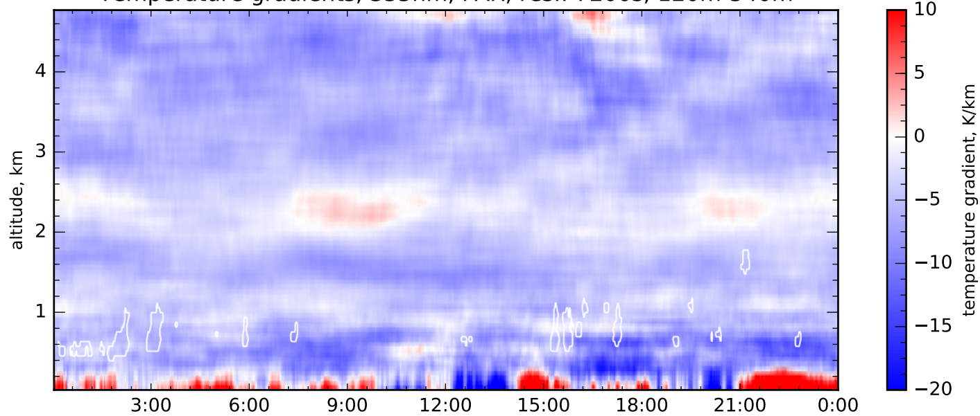
Temperature gradients, 355nm, FAR, res.: 7200s, 120m-540m
