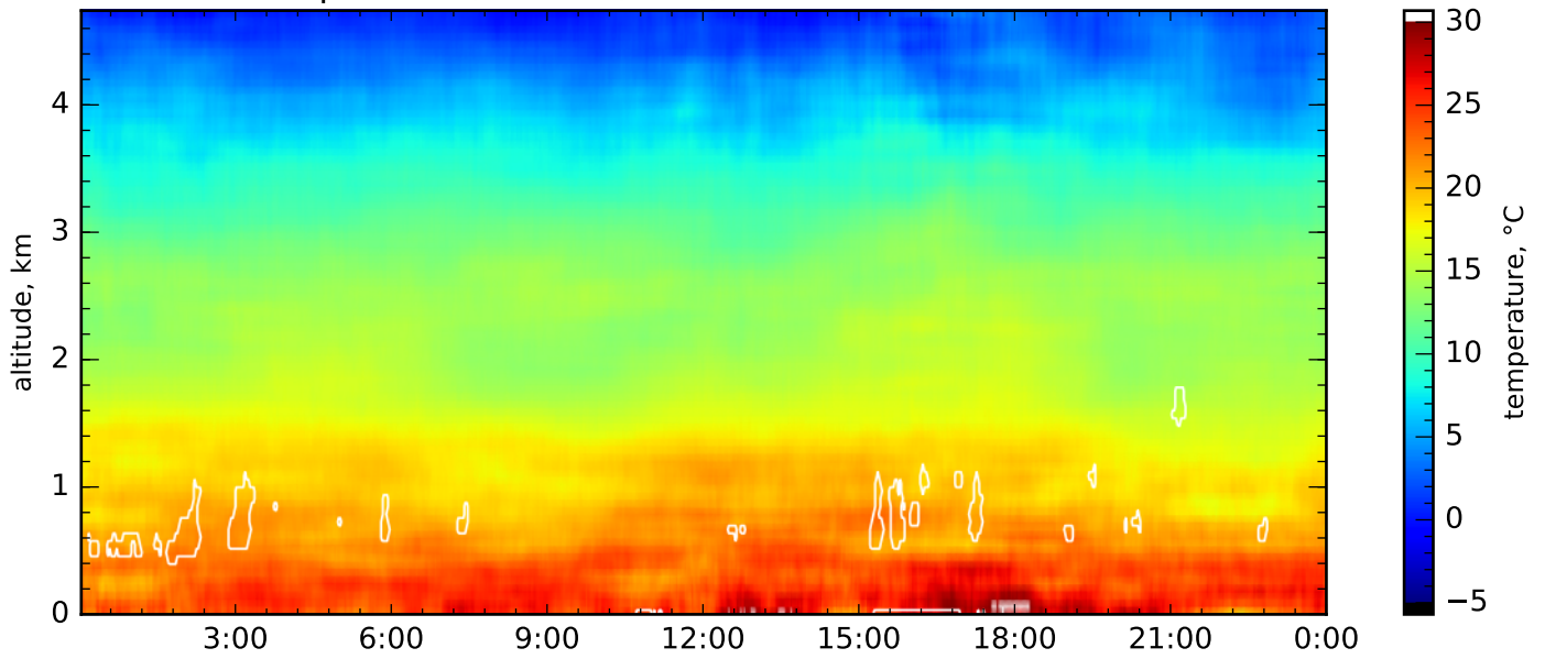
Temperature, 355nm, FAR, res.: 7200s, 120m-540m
