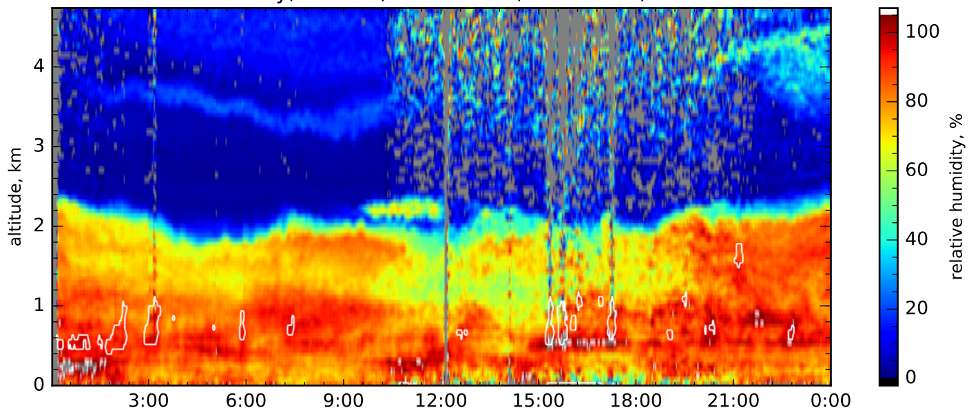
Relative humidity, 355nm, FAR+NEAR, res.: 600s, 120m-540m
