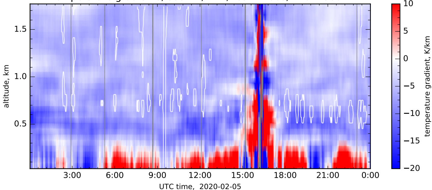
Temperature gradients, 355nm, FAR, res.: 7200s, 120m-300m
