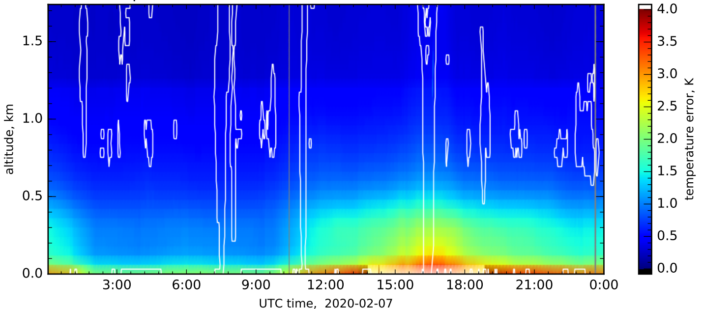
Temperature error, 355nm, FAR, res.: 7200s, 120m-300m
